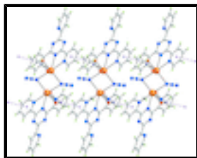
Fig. 2. Supramolecular chains in (I) mediated by \pi \cdots \pi interactions shown as purple dashed lines.
